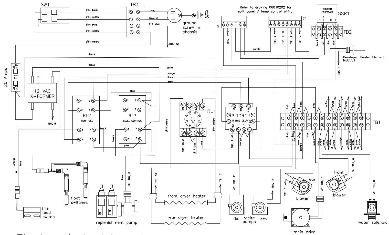
Fischer Industries, Inc. 3000S, 3000ST, 4000M Wiring Diagram, 110 VAC Drawing No. 06030200 rev. 1 03/14/07
